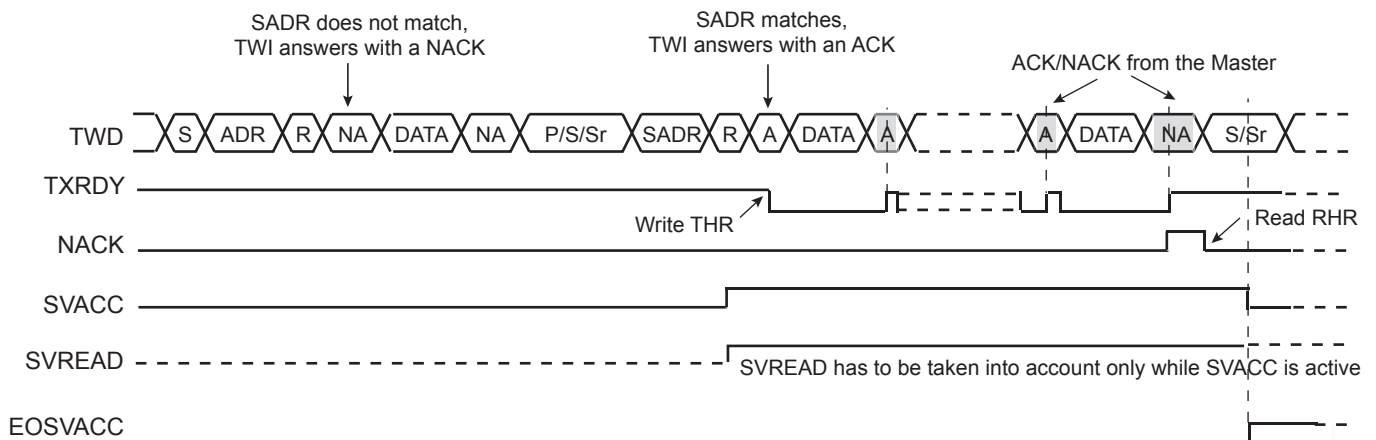
Figure 29-26. Read Access Ordered by a MASTER
