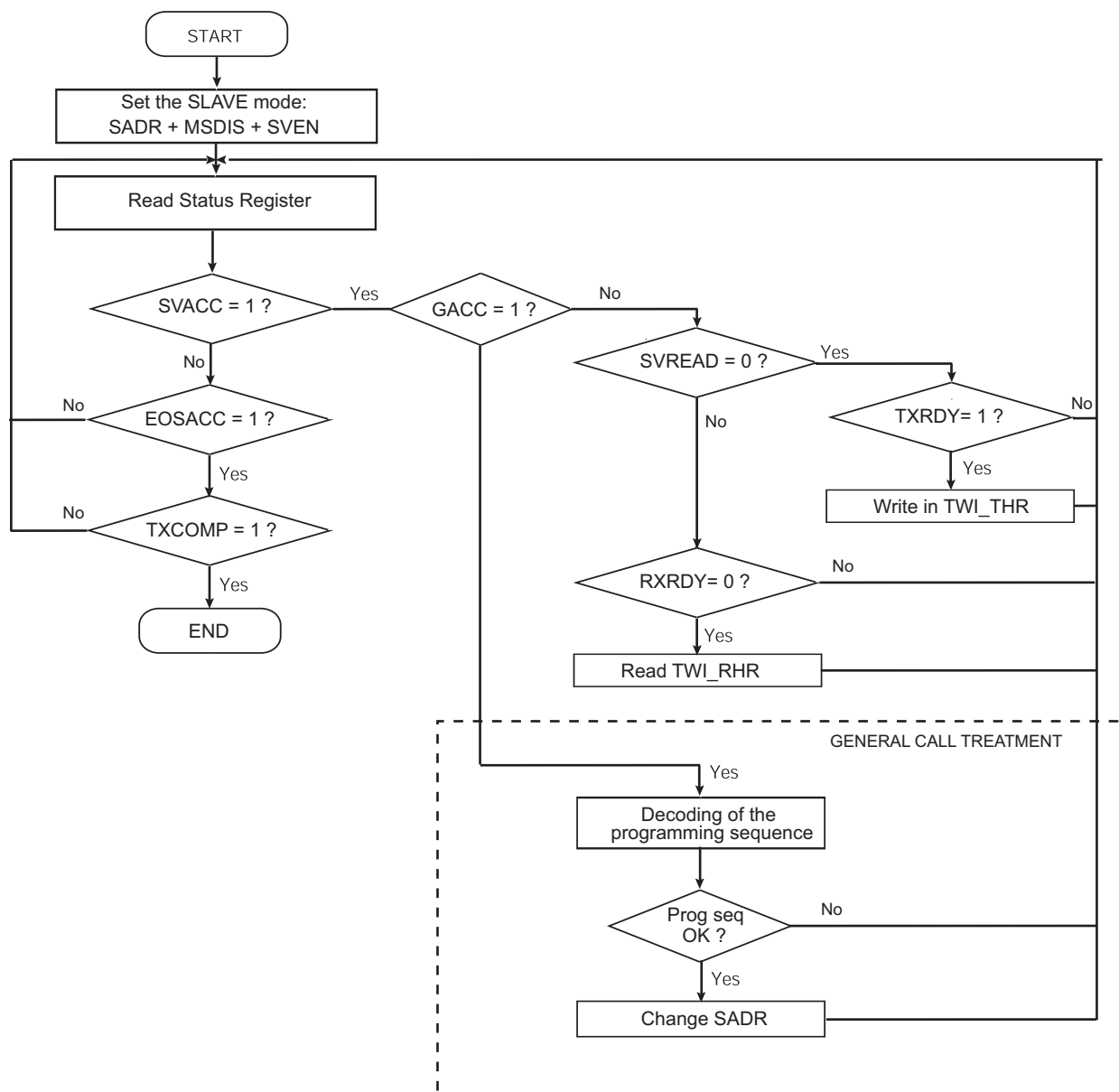
Figure 29-33. Read Write Flowchart in Slave Mode
