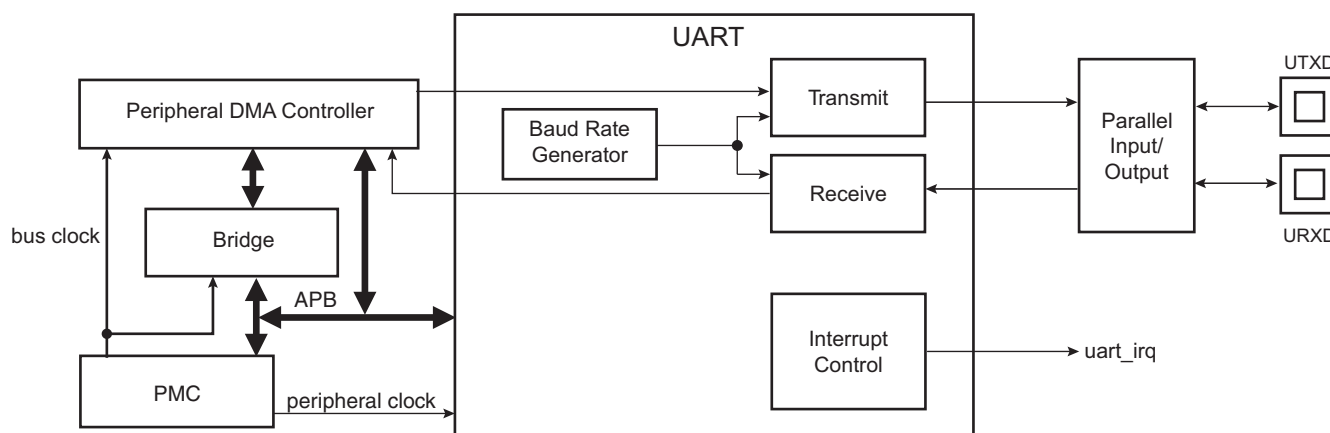
Figure 32-1. UART Block Diagram
