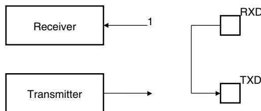
Figure 33-28. Remote Loopback Mode Configuration
