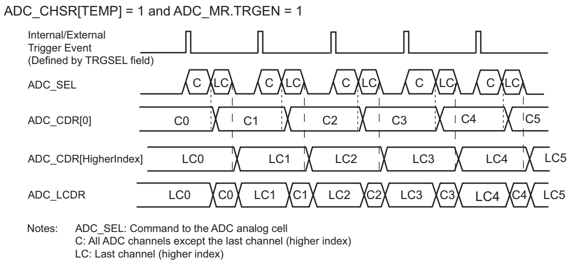
Figure 35-6. Same Trigger for All Channels
