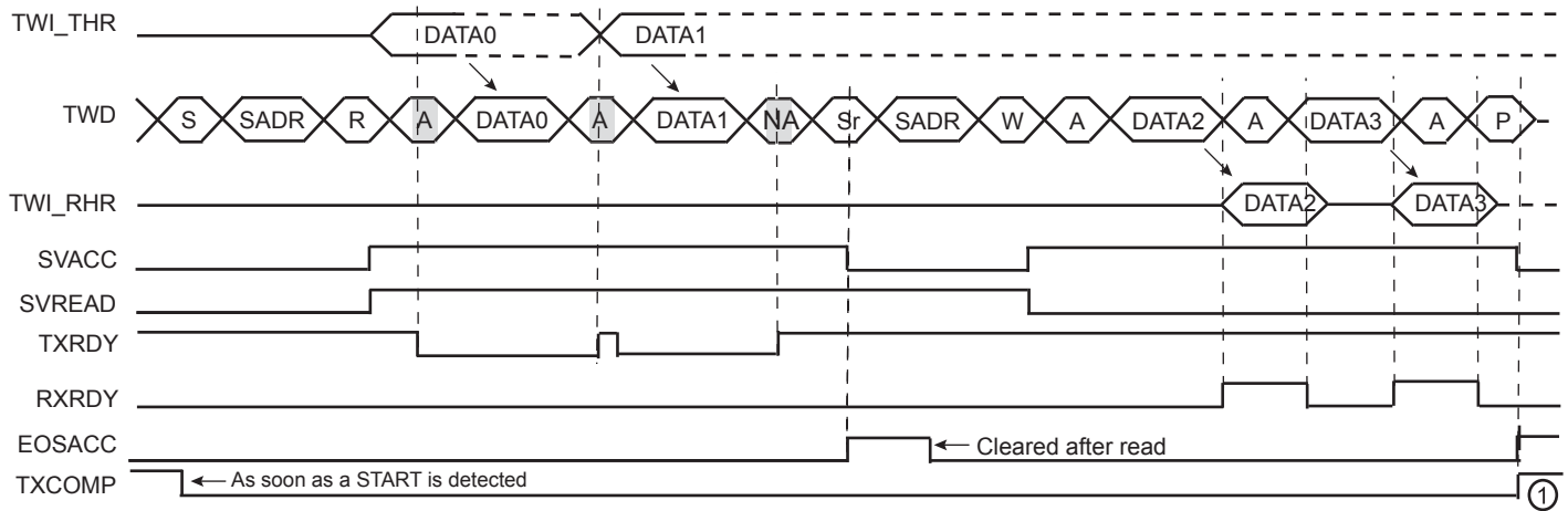
Figure 29-31. Repeated Start + Reversal from Read to Write Mode
