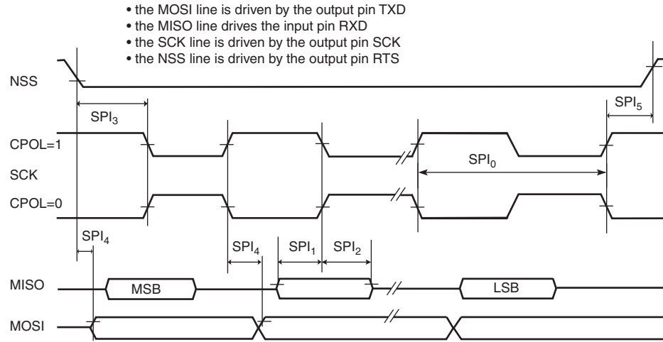
Figure 36-15. USART SPI Master Mode
