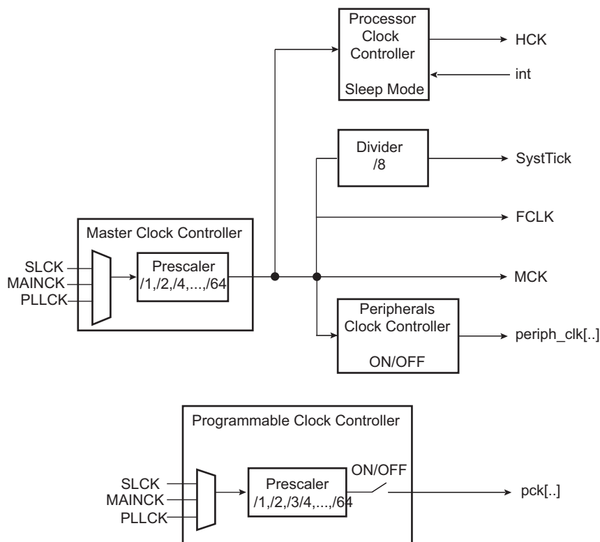
Figure 9-2. SAM G53 Power Management Controller Block Diagram
