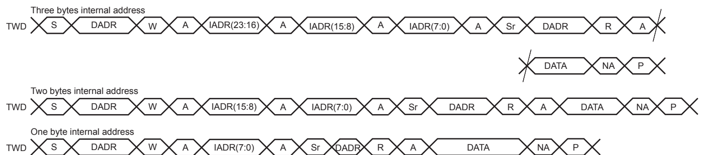
Figure 29-13. Master Read with One, Two or Three Bytes Internal Address and One Data Byte
