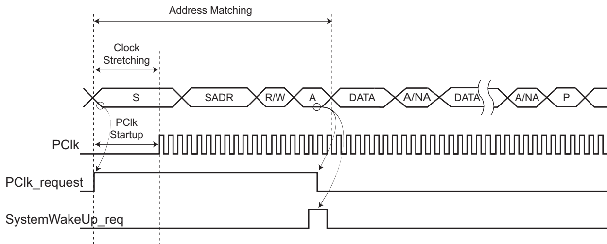
Figure 28-44. Address Match and Data Matching Disabled
