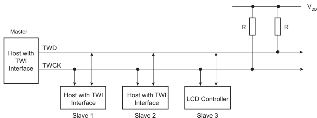
Figure 29-25. Slave Mode Typical Application Block Diagram
