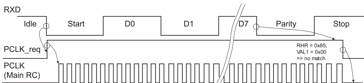
Figure 32-13. Asynchronous Event Generating Only Partial Wake-up
