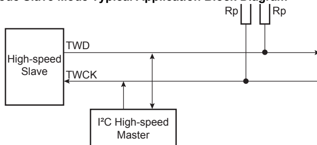
Figure 28-34. High-Speed Mode Slave Mode Typical Application Block Diagram
