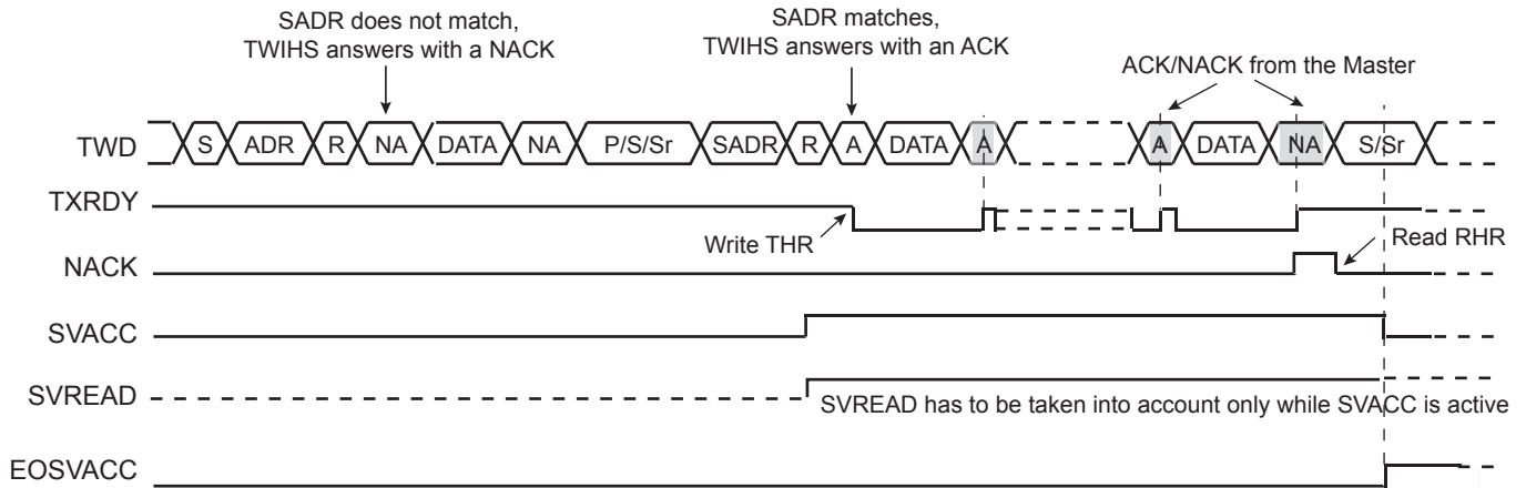
Figure 28-36. Read Access Ordered by a Master
