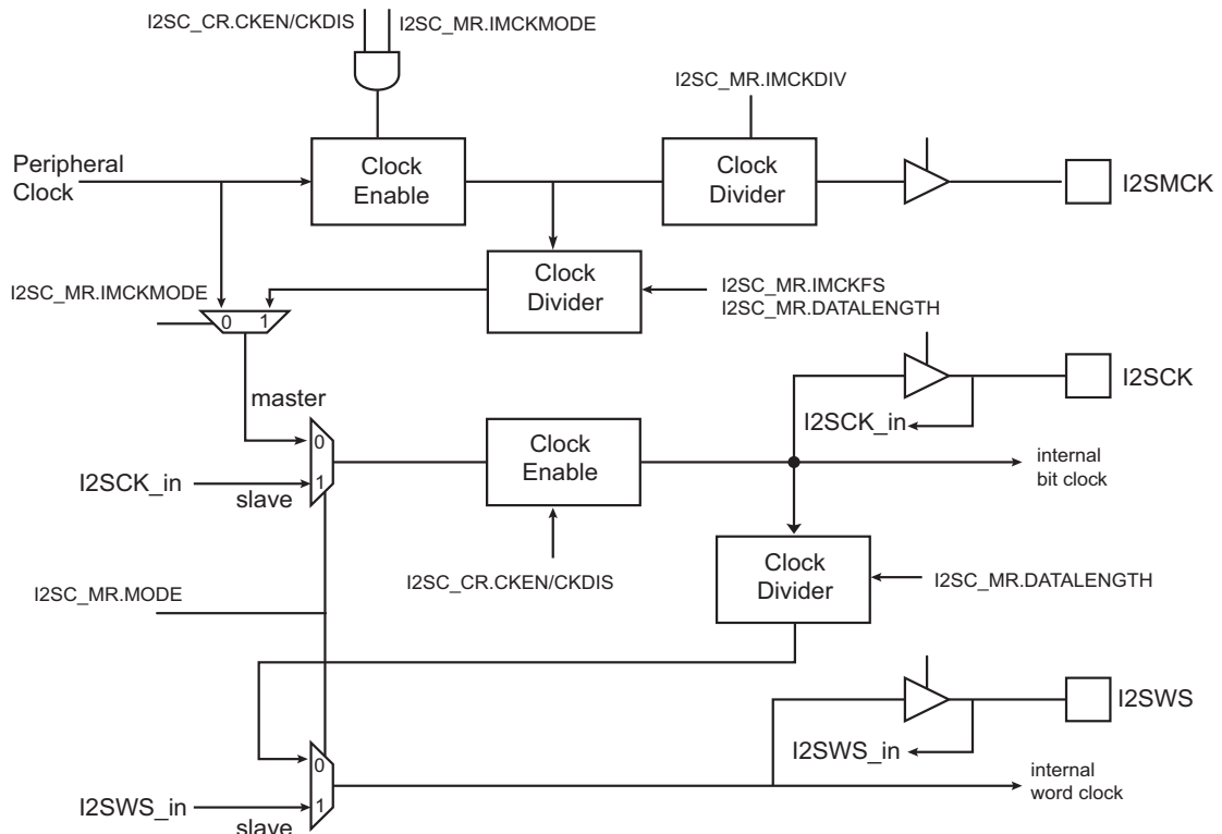
Figure 30-3. I2SC Clock Generation
