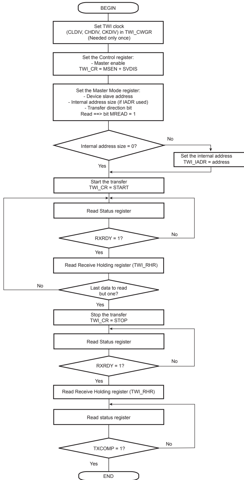
Figure 29-21. TWI Read Operation with Multiple Data Bytes with or without Internal Address
