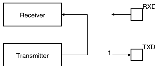
Figure 33-27. Local Loopback Mode Configuration
