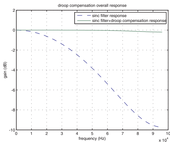
Figure 31-5. Droop Compensation Filter Overall Frequency Response
