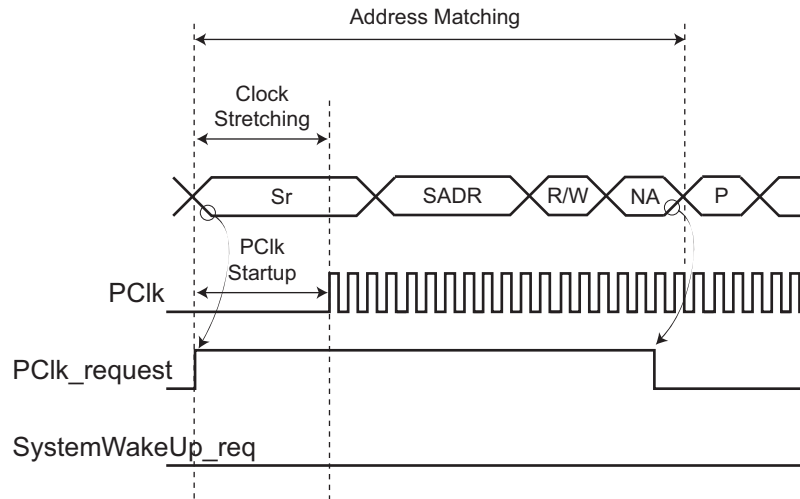
Figure 28-45. No Address Match and Data Matching Disabled
