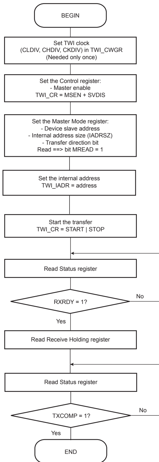
Figure 29-20. TWI Read Operation with Single Data Byte and Internal Address
