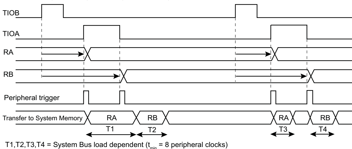
Figure 34-5. Example of Transfer with PDC
