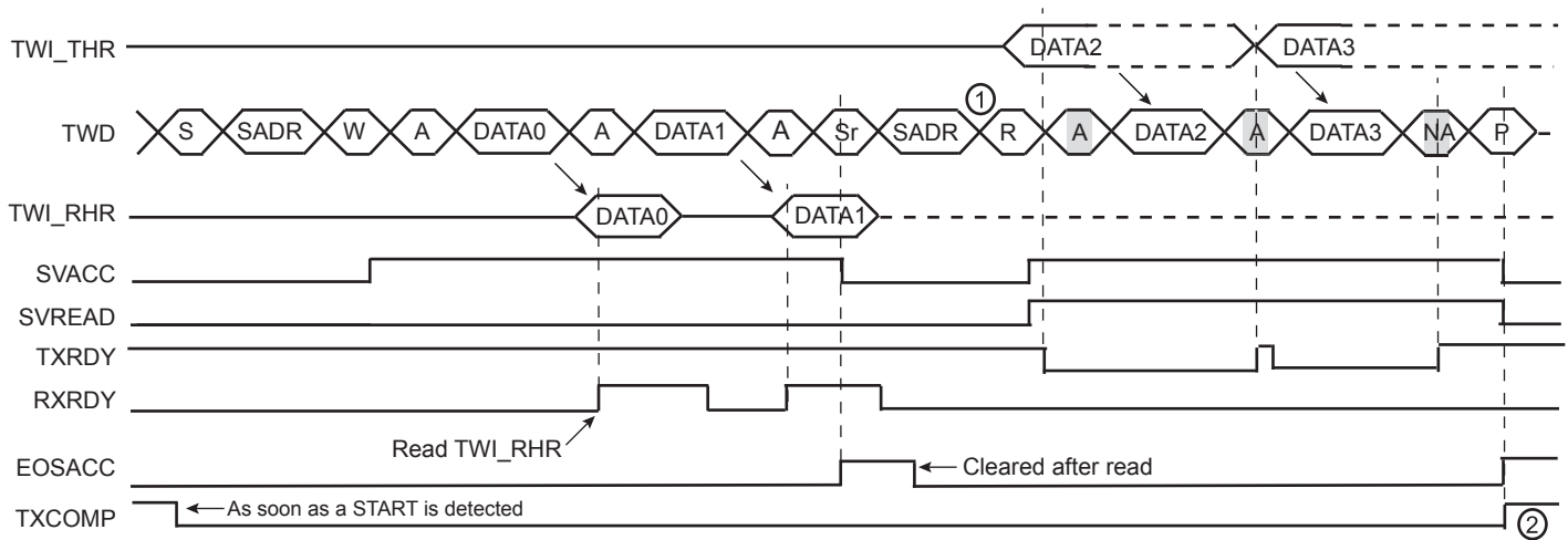
Figure 29-32. Repeated Start + Reversal from Write to Read Mode
