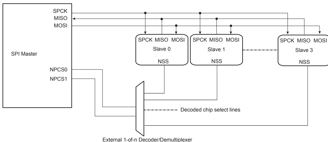
Figure 27-10. Chip Select Decoding Application Block Diagram: Single Master/Multiple Slave Implementation
