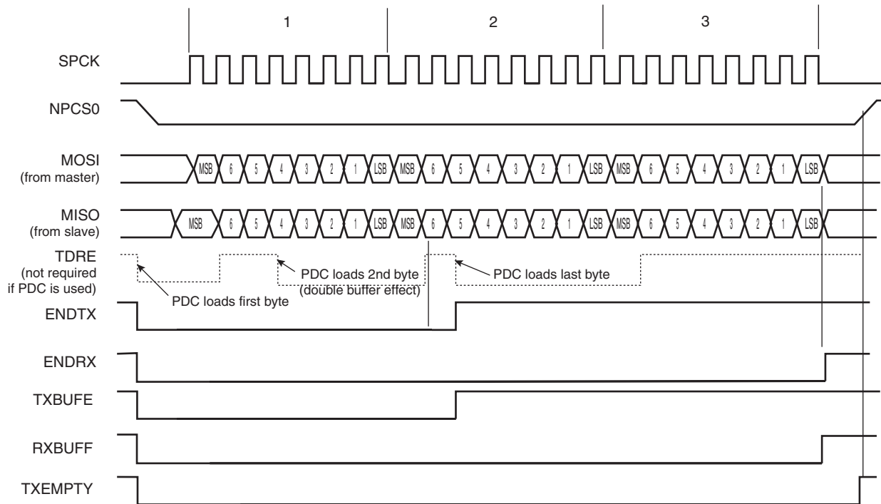
Figure 27-8. PDC Status Register Flags Behavior
