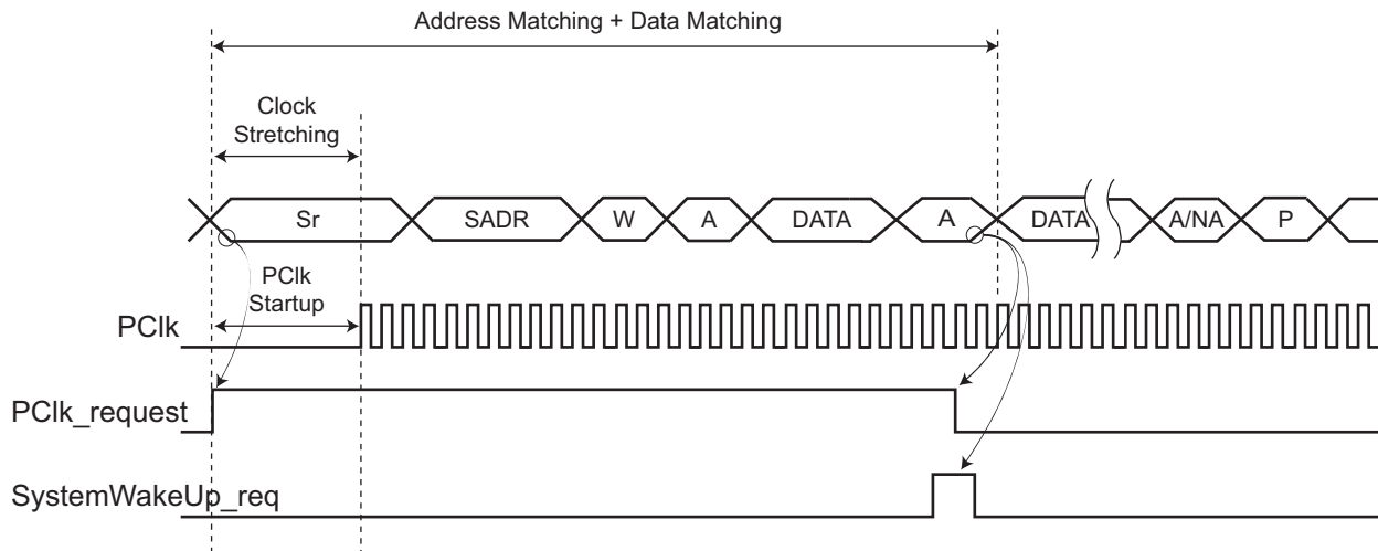
Figure 28-46. Address and Data Match (Data Matching Enabled)
