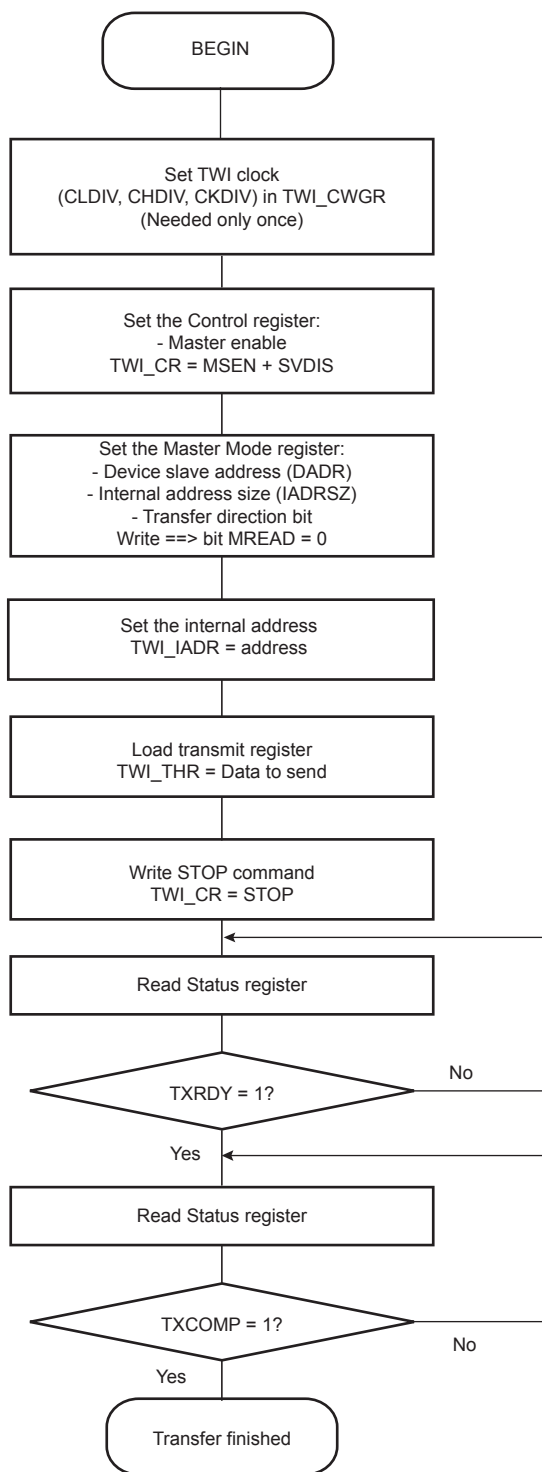
Figure 29-17. TWI Write Operation with Single Data Byte and Internal Address
