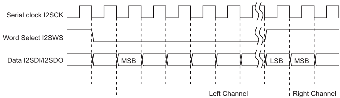
Figure 30-2. I 2 S Reception and Transmission Sequence
