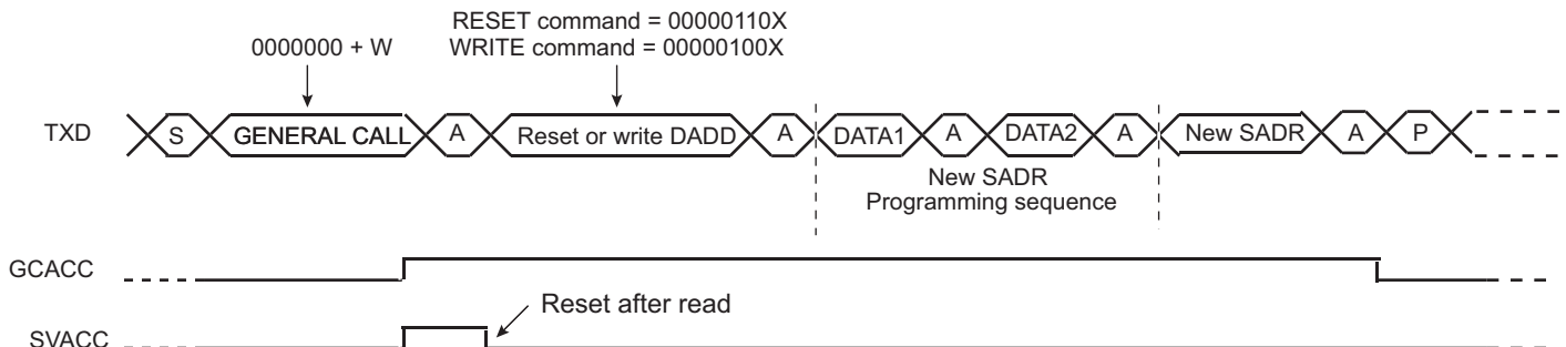
Figure 29-28. Master Performs a General Call
