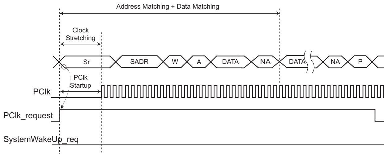
Figure 28-47. Address Matches and Data Do Not Match (Data Matching Enabled)
