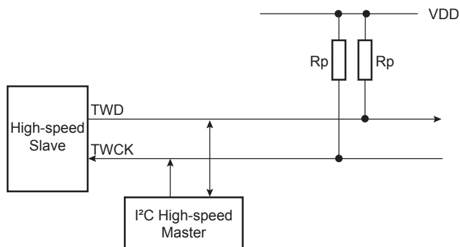
Figure 28-2. High-Speed Mode Application Block Diagram
