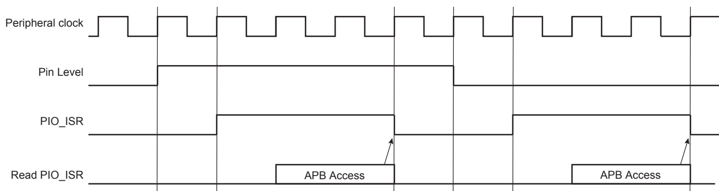
Figure 26-8. Input Change Interrupt Timings When No Additional Interrupt Modes
