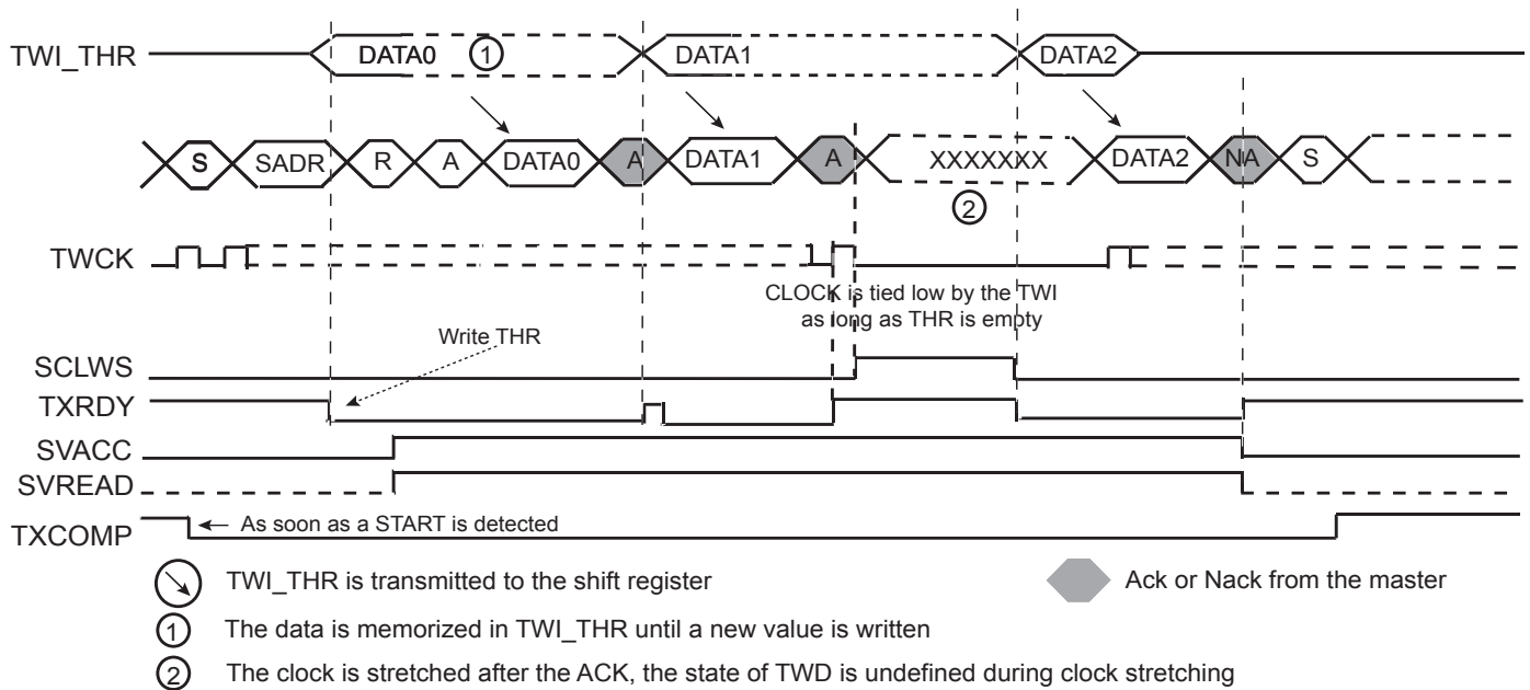
Figure 29-29. Clock Stretching in Read Mode
