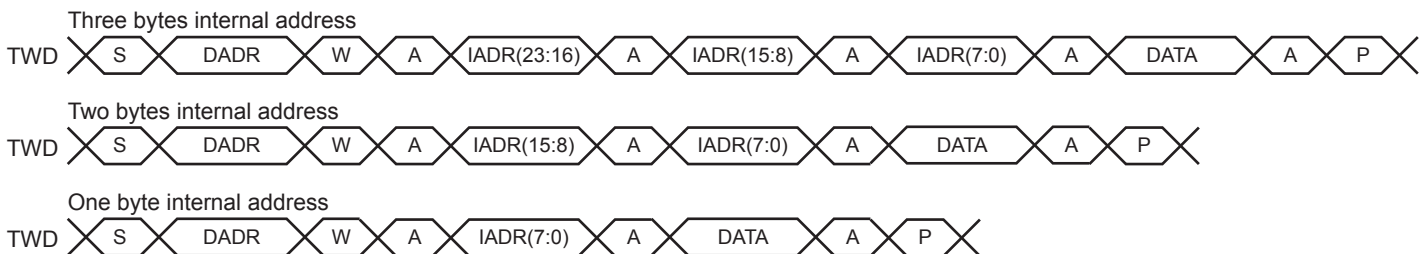
Figure 29-12. Master Write with One, Two or Three Bytes Internal Address and One Data Byte
