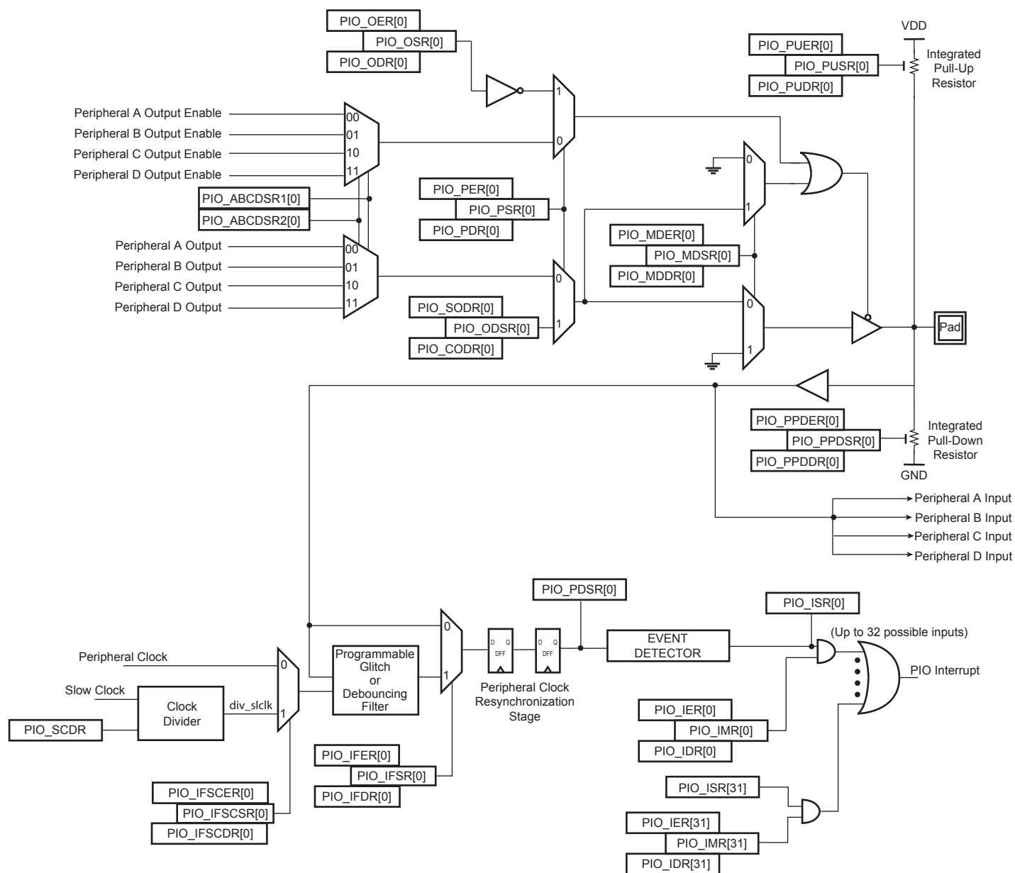
Figure 26-3. I/O Line Control Logic
