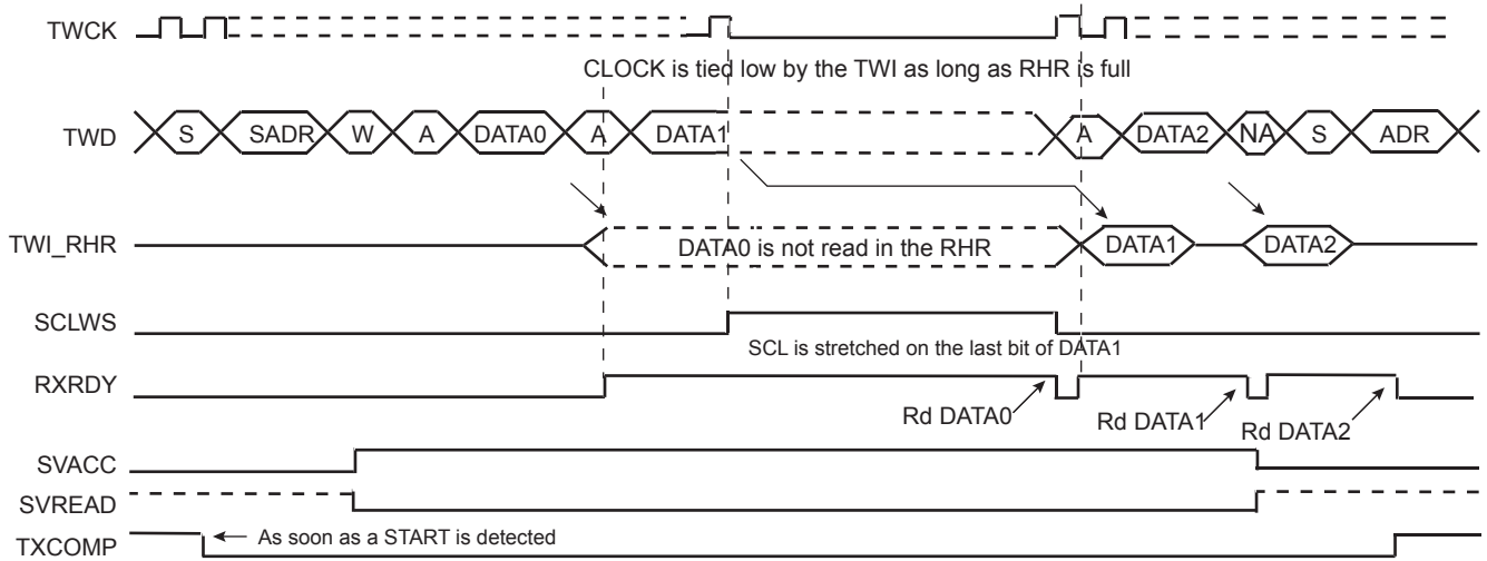
Figure 29-30. Clock Synchronization in Write Mode
