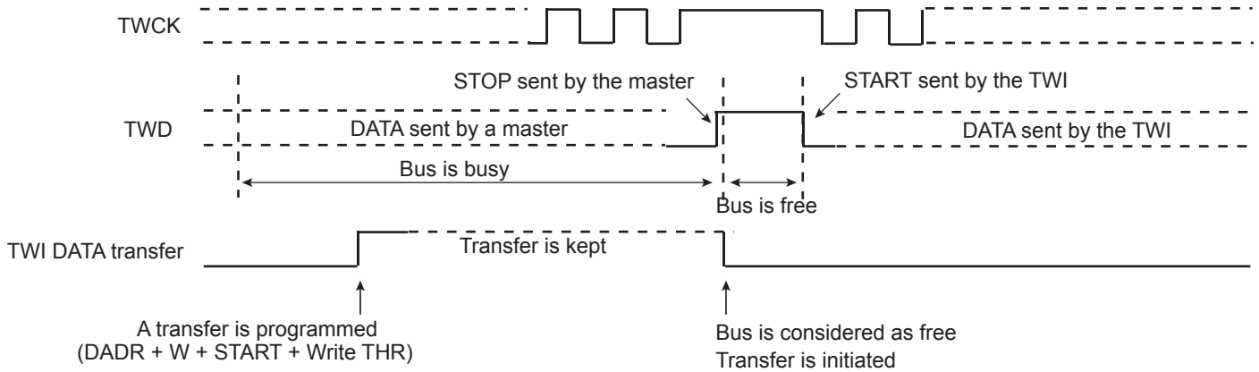
Figure 29-22. Programmer Sends Data While the Bus is Busy
