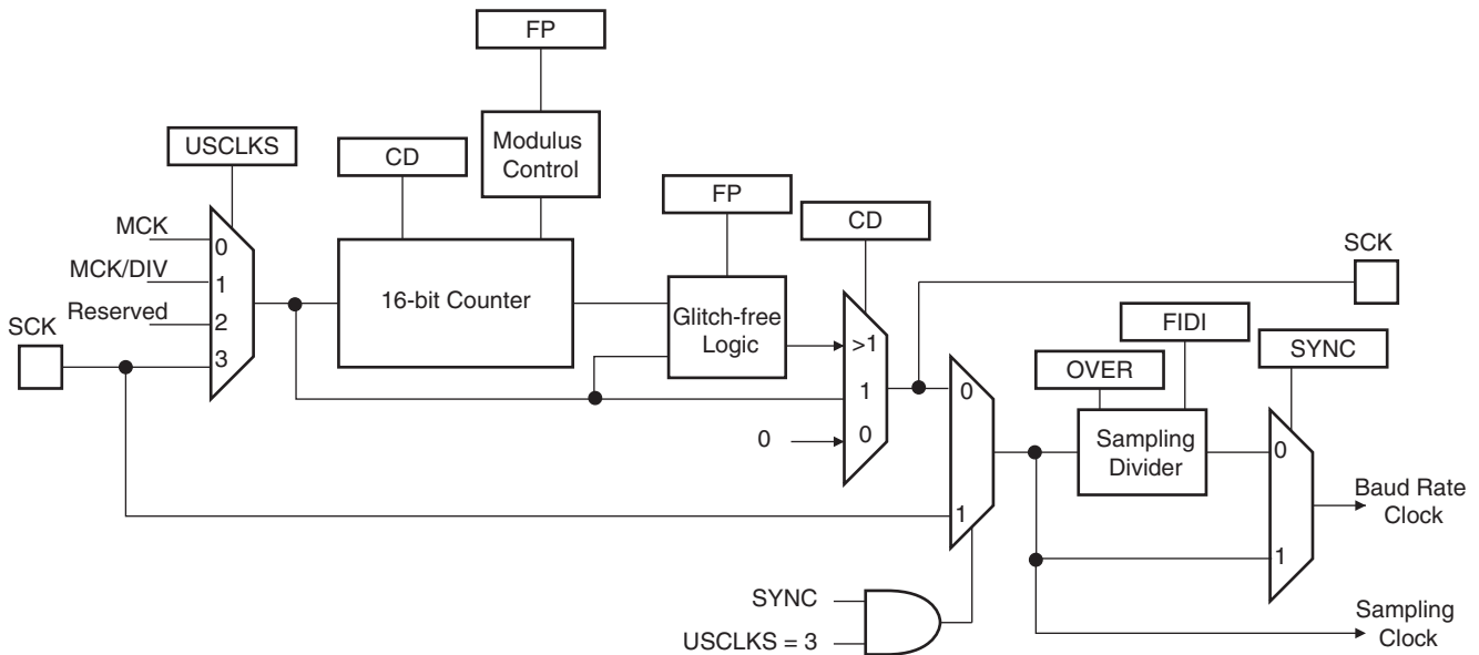
Figure 33-3. Fractional Baud Rate Generator
