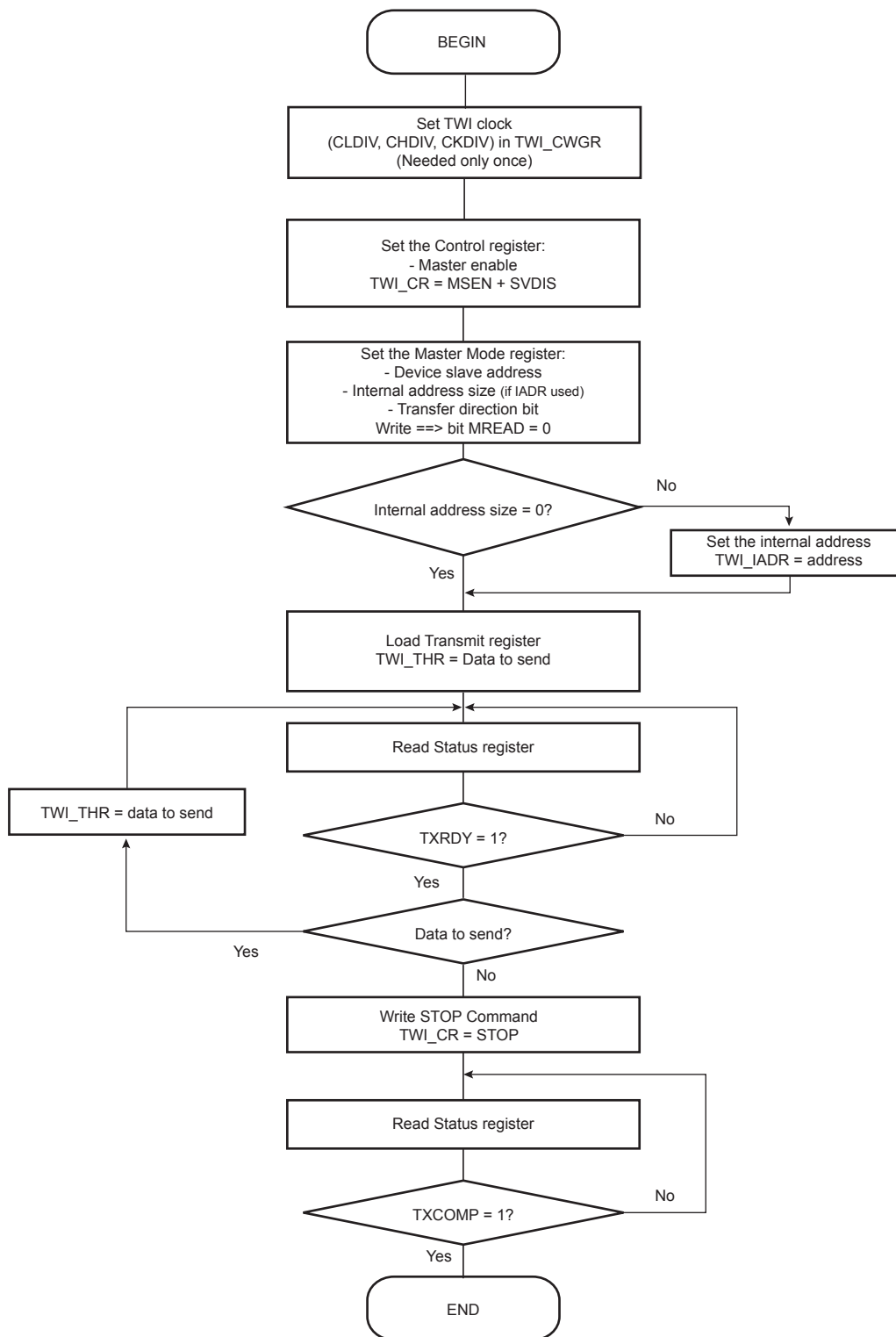
Figure 29-18. TWI Write Operation with Multiple Data Bytes with or without Internal Address
