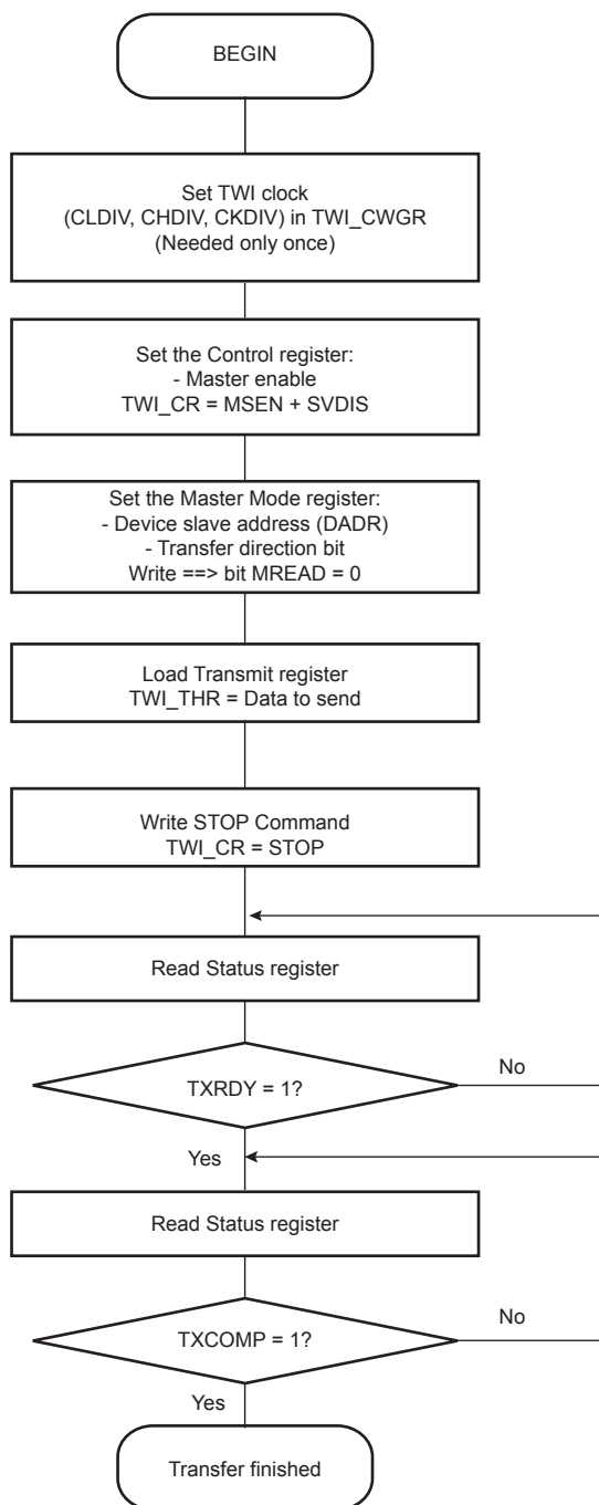
Figure 29-16. TWI Write Operation with Single Data Byte without Internal Address
