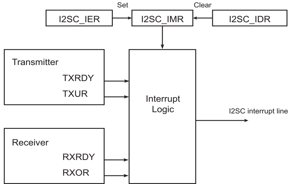
Figure 30-4. Interrupt Block Diagram
