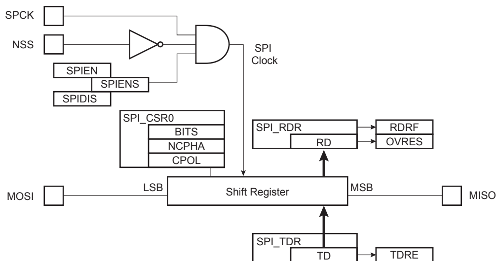
Figure 27-12. Slave Mode Functional Block Diagram
