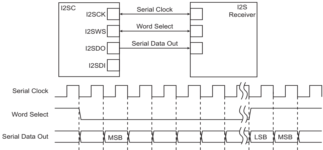
Figure 30-5. I2SC Application Example
