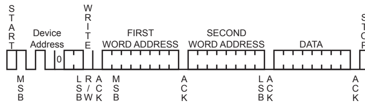
Figure 29-14. Internal Address Usage
