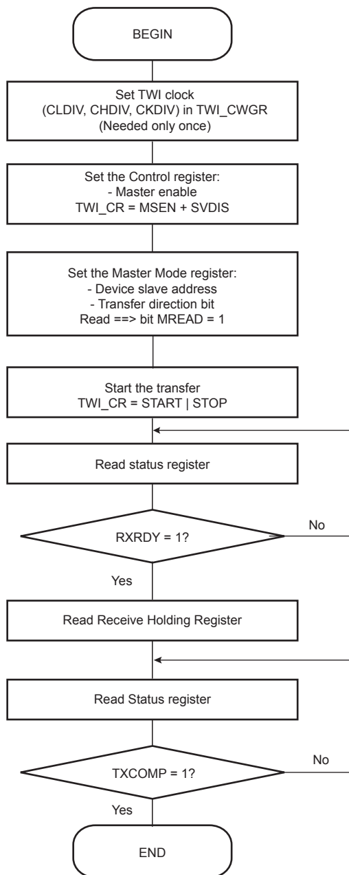
Figure 29-19. TWI Read Operation with Single Data Byte without Internal Address
